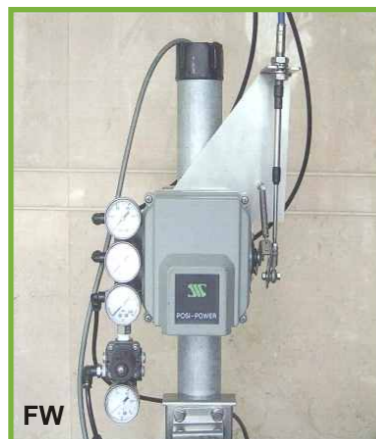
Wire Positioner
